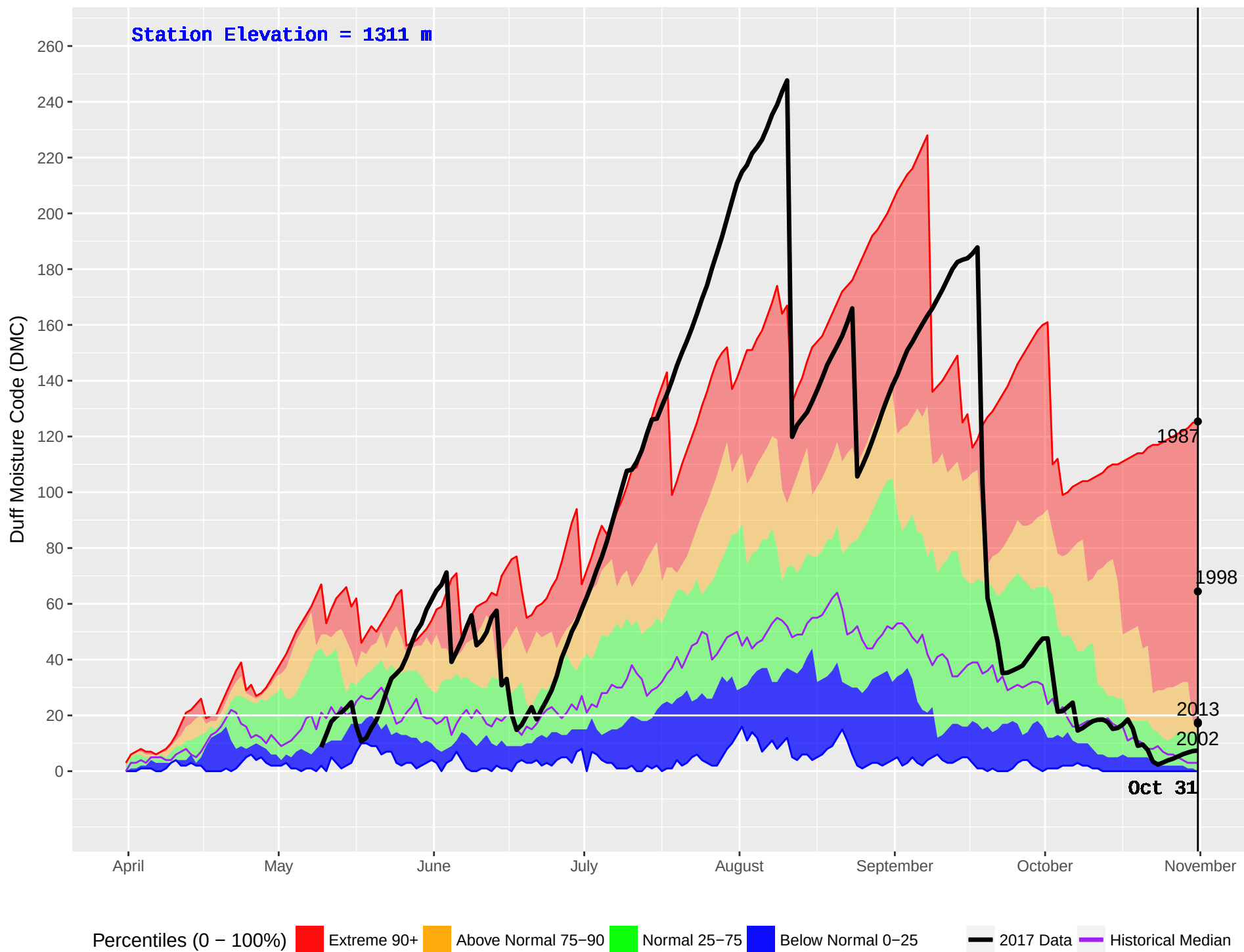
FLATHEAD 2 (418) : Historical (1986–2016) and Current (2017) Noon Duff Moisture Code (DMC)
